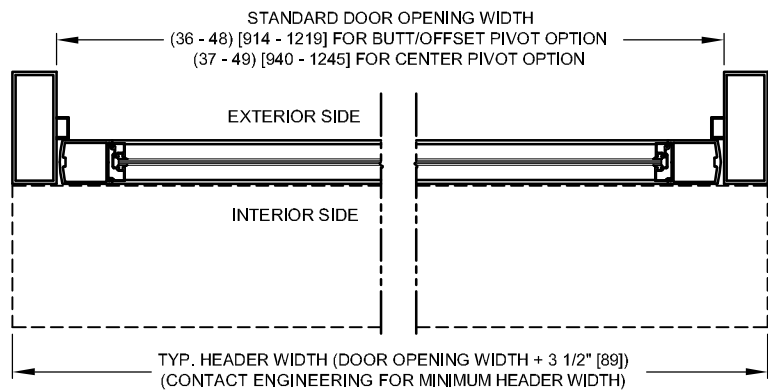
HORIZONTAL SECTION
