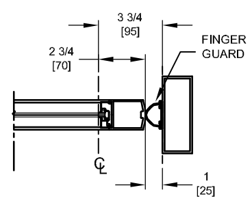
HINGE JAMB AT CENTER PIVOT OPTION
